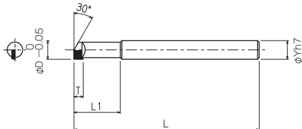
TYPE I 1枚刃 1 flute
