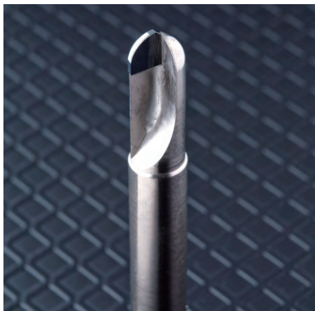
1枚刃 1 flute
