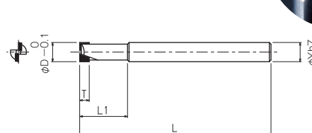
TYPE II 2枚刃 2 flute
